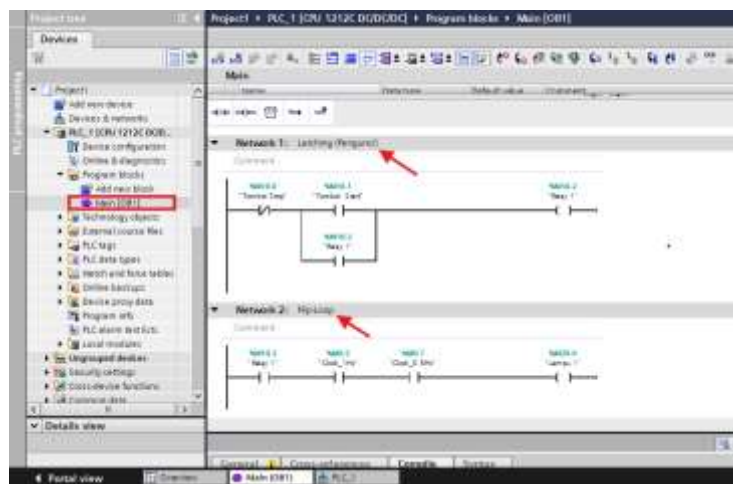
Gambar 2. 7 Add New Block Main [OB1]
