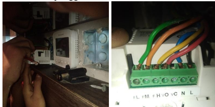
Gambar 9 Wired Remote Control
