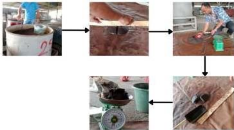
Gambar 2.11 proses sampling
