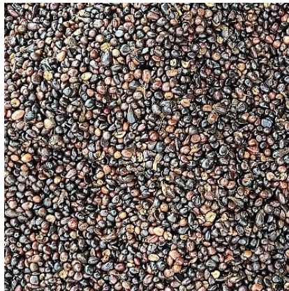
Gambar 1.6 Kernel
