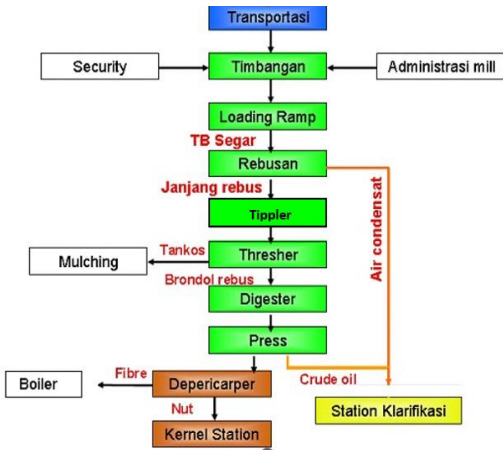
Gambar 1.4 Diagram proses pengolahan kelapa sawit
