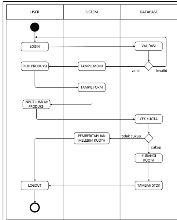
Gambar 2.1 Activity Diagram Produksi
