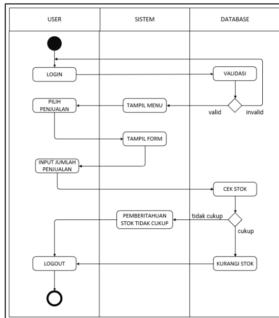
Gambar 2.2 Activity Diagram Penjualan
