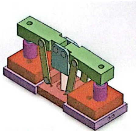
Gambar 2. 9 Pneumatic Double Clamp Cylinder
