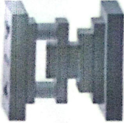
Gambar 2. 14 Dies Blanking
