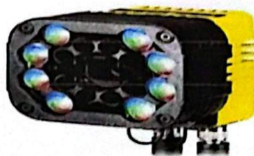
Gambar 1.6 In-Sight 3800 Vision System
