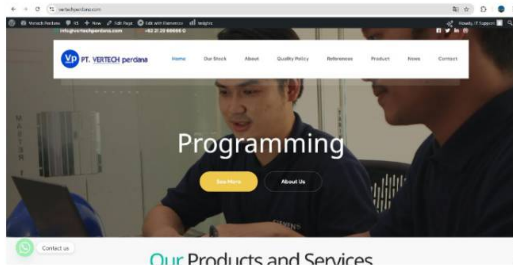
Gambar 2. 1 Tampilan Website
