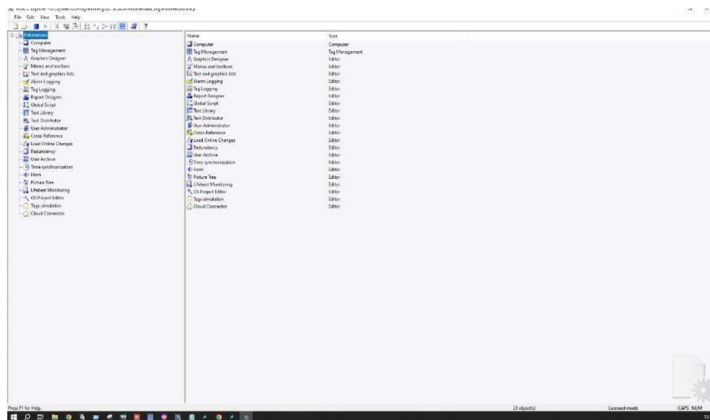
Gambar 2.2 Graphics Manager
